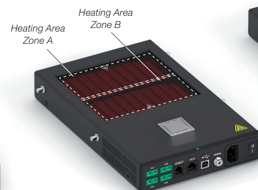
PHNE Preheater for PCBs up to 11 x 7 cm / 4 x 3"
