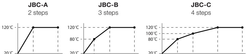
Profiles set using the low position of the PHXL-SA Support (28 mm in height between the PCB and the heating area).
